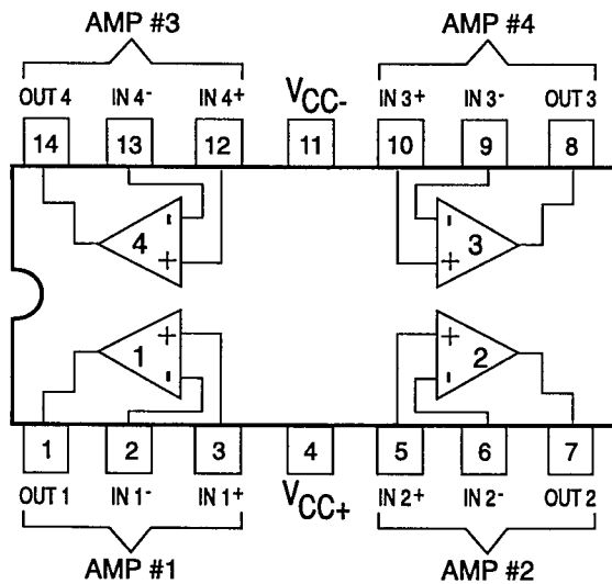
IC1162 &amp; IC1052 (TL074) QUAD OP-AMP
