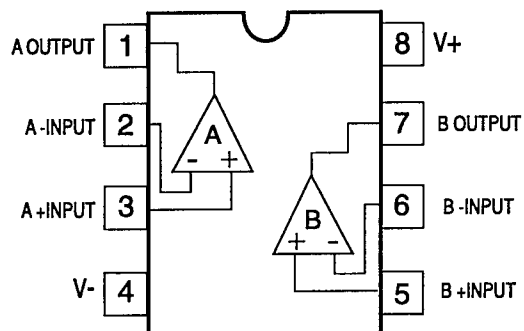
IC1175 (NJM5532), IC1041 (TL072) DUAL OP-AMP
